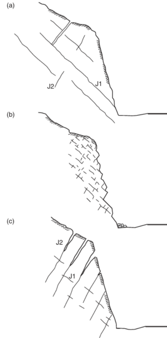
Slope failure
